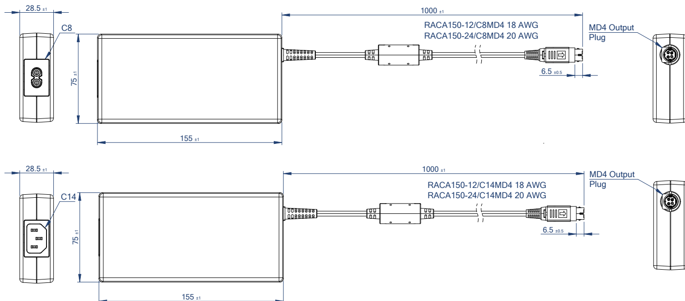
Dimension Drawing RACA150 (mm)
