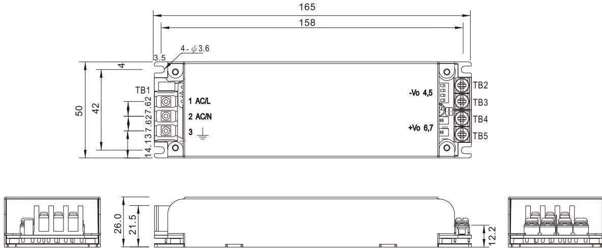
AC Input Terminal(TB1) pin NO. Assignment
