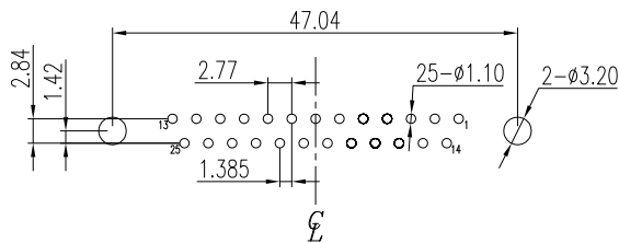
RECOMMENDED P.C.B LAYOUT INSPECTION DIMENSION:(A)~(F)
