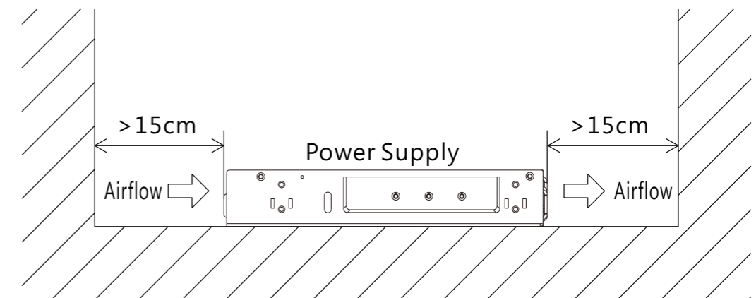
Figure 3-1 Mounting Diagram
