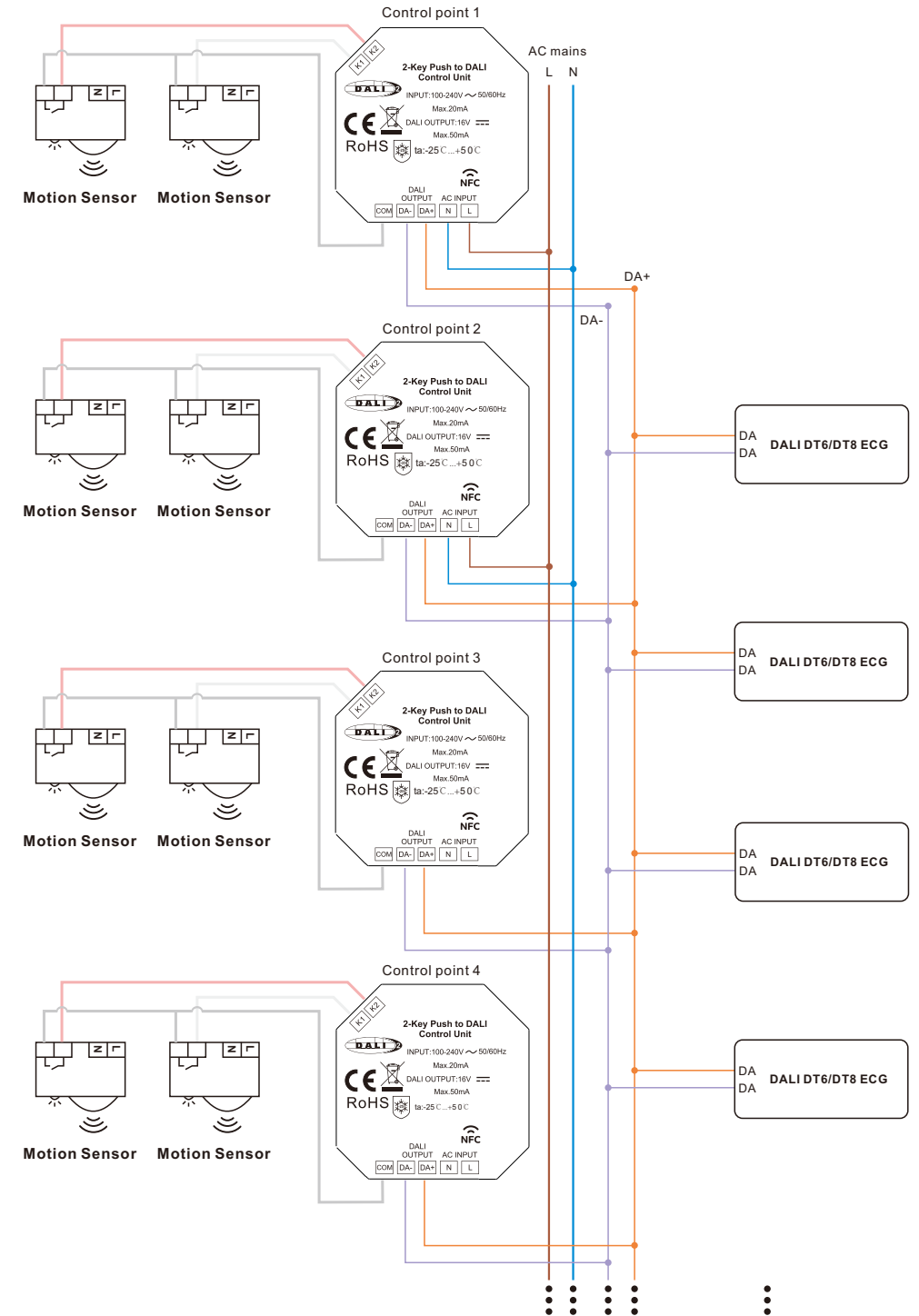
Figure 2: Wiring scheme to control up to 50 DALI ECGs (2 control units powered by AC mains, the other 2 powered by DALI bus)
