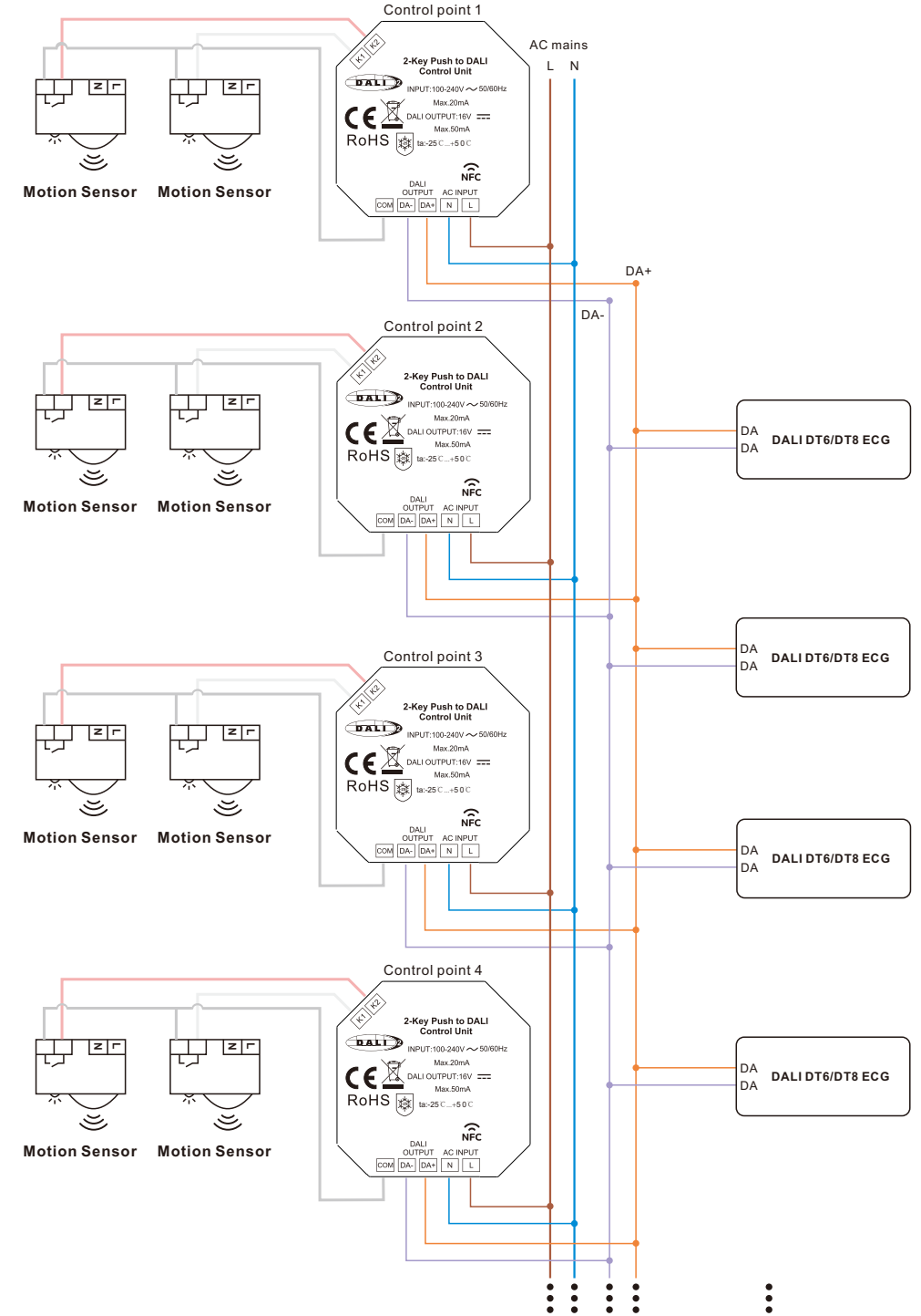
Figure 4: Wiring scheme to control up to 100 DALI ECGs (all 4 control units powered by AC mains)
