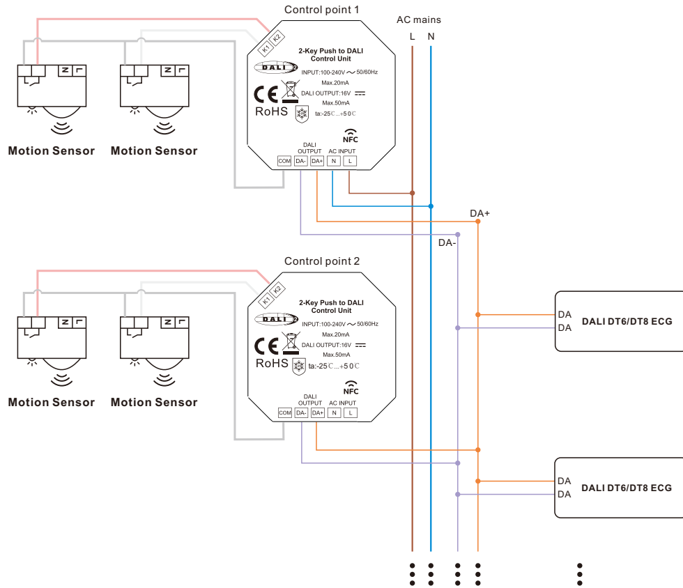
Figure 1: Wiring scheme to control up to 25 DALI ECGs (only 1 control unit powered by AC mains, the other powered by DALI bus)
