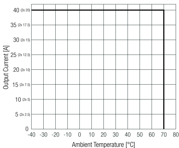
Derating Graph
