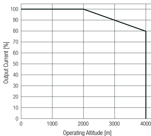
Altitude Derating
