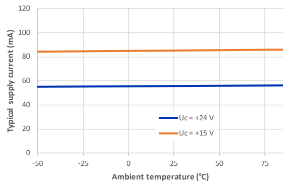
Figure 3: Supply current function of temperature
