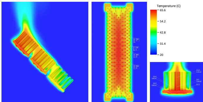
Single fan solution
