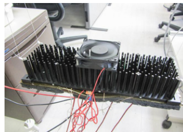
Single fan solution
