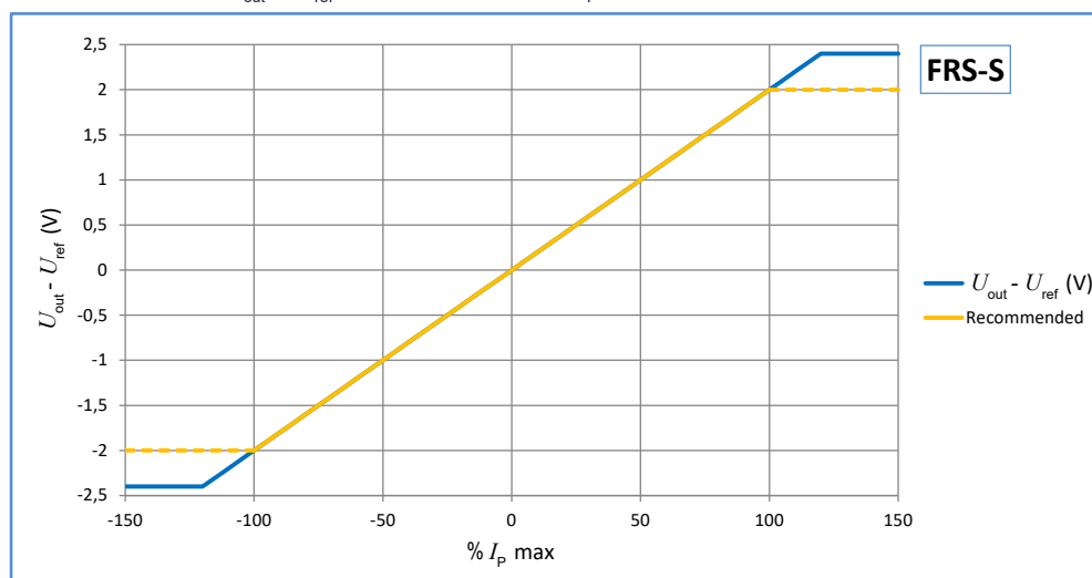
Figure 1: Bi-polar output voltage ( U_{\text{out}} - U_{\text{ref}} ) VS primary current I_P
