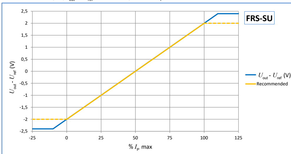
Figure 2: Uni-polar output voltage ( U_{\text{out}} - U_{\text{ref}} ) VS primary current I_P
