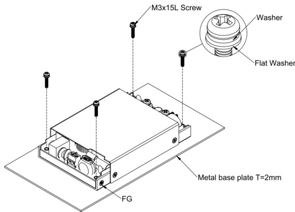
LFM550SXXXC Installation Diagram
