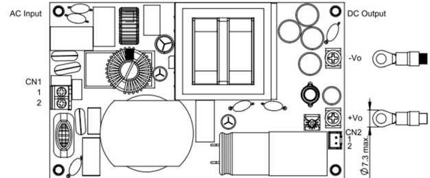
LFM550SXXXB Installation Diagram
