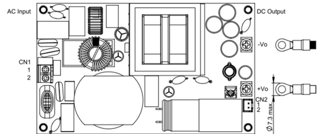
LFM550SXXXC Installation Diagram
