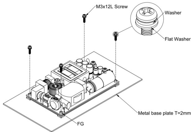
LFM550MXXXB Installation Diagram
