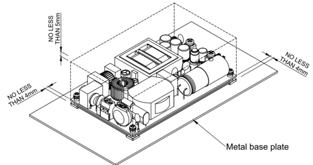
LFM550MXXXB Installation Diagram
