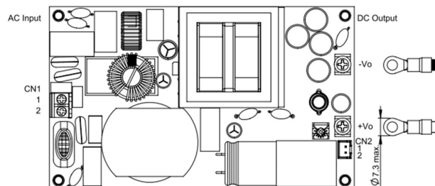
LFM550MXXXB Installation Diagram
