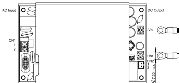
LFM550MXXXC Installation Diagram
