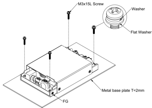
LFM550MXXXC Installation Diagram
