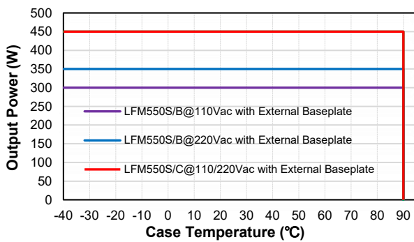
Output Power vs Case Temperature ( T_c )
