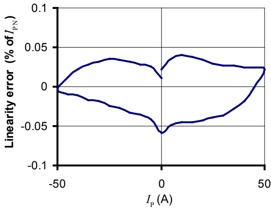
Figure 7: Linearity error
