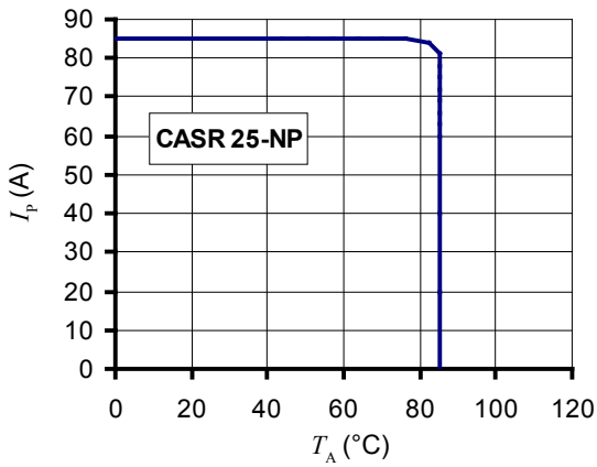
Figure 13: I_p vs T_A for CASR 25-NP/SP1
