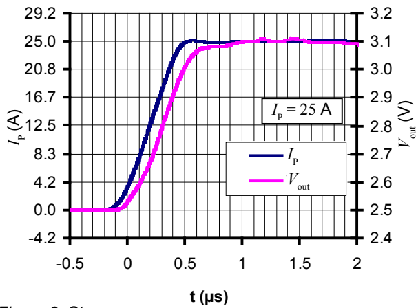
Figure 3: Step response
