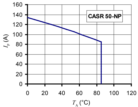
Figure 14: I_p vs T_A for CASR 50-NP/SP1
