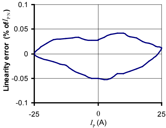
Figure 1: Linearity error
