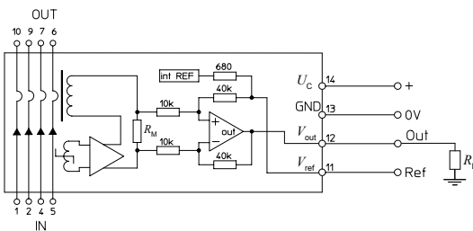
Figure 17: Test connection
