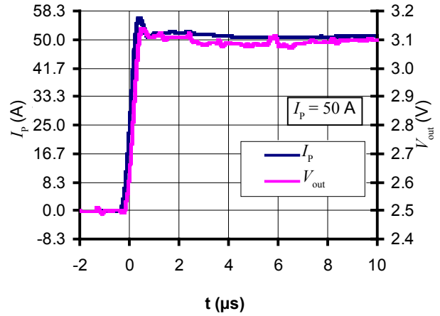
Figure 10: Step response
