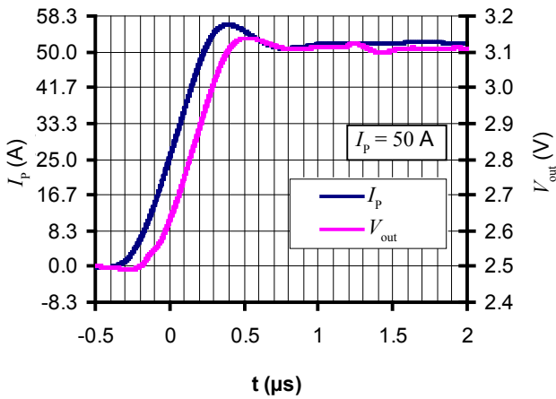
Figure 9: Step response
