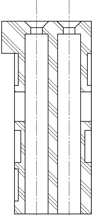
SECTION X-X' (6/1)
