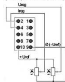
Program Input Connections (Example with external pot)
