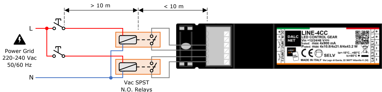
Figure 7: Connecting the Local Command for Long Distances
