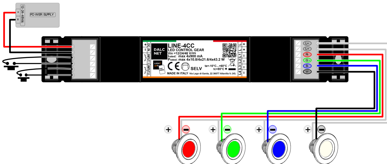
Figure 5: Wiring diagram for RGBW LED load
