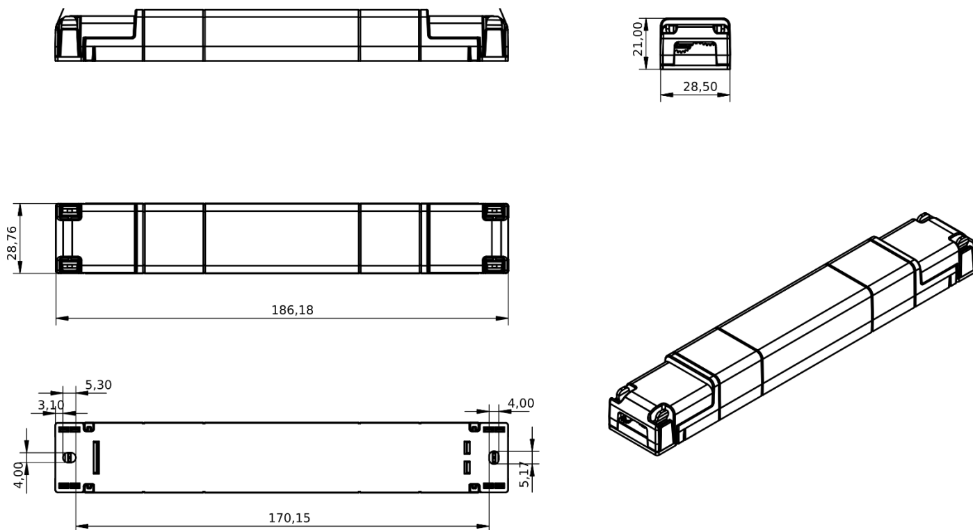
Figure 12: Dimensions and mechanical dimensions
