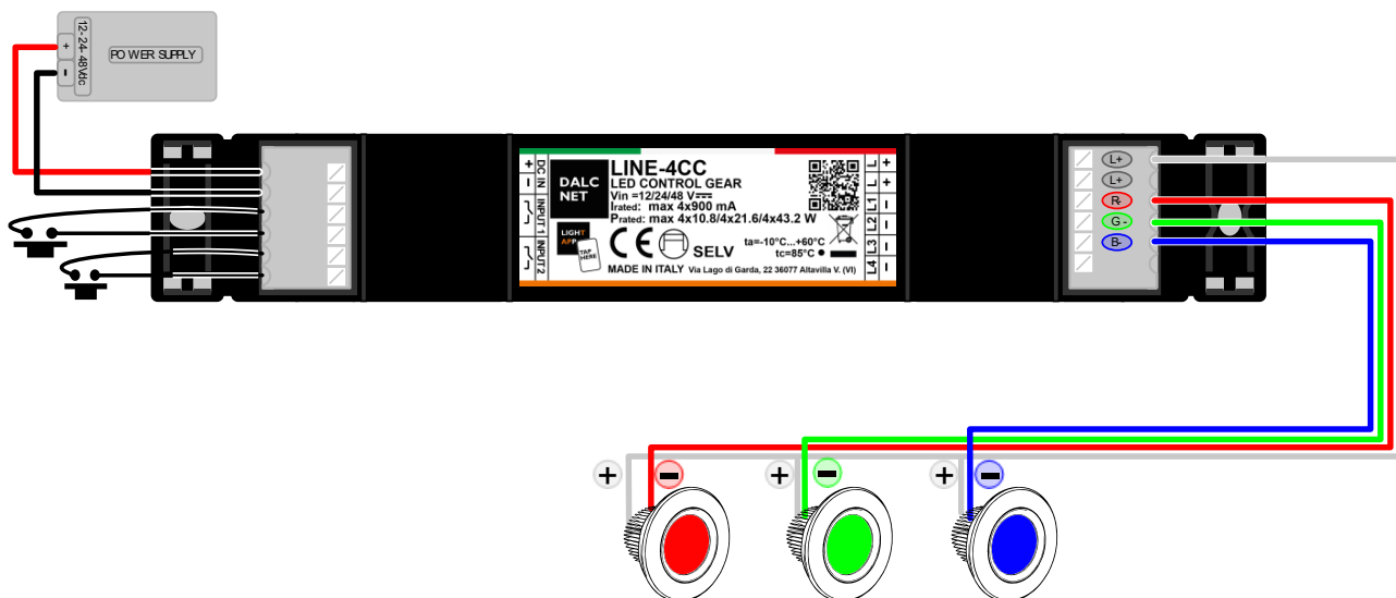
Figure 4: Wiring diagram for RGB load
