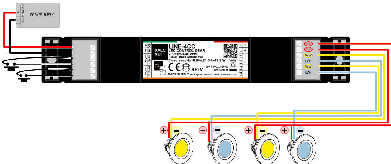
Figure 3: Wiring Diagram for Tunable-White LED Loads
