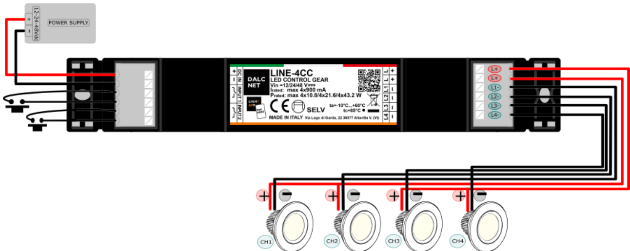
Figure 2: Wiring diagram for White or Monochrome LED loads
