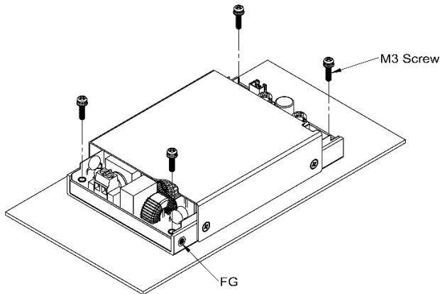
LFM420MXXC Installation Diagram
