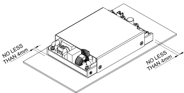
LFM420MXXC Installation Diagram
