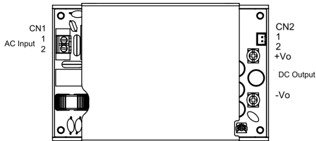
LFM420MXXXC Installation Diagram
