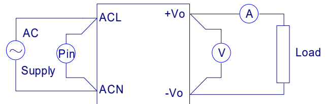
Figure 1. LFM300M Series Test Setup
