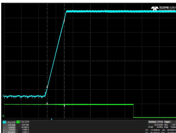
Figure 15: LCC600-12H-9P Output Startup Characteristic
