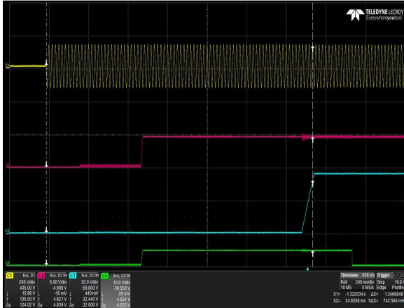
Figure 41: LCC600-36U-9P Turn-on delay via AC mains
