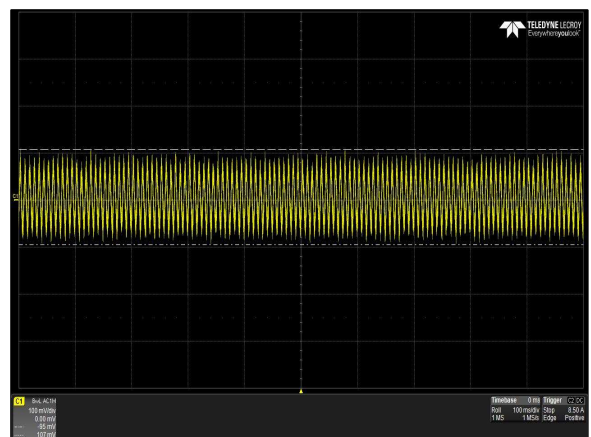
Figure 76: LCC600-48H-9P Ripple and Noise Measurement
