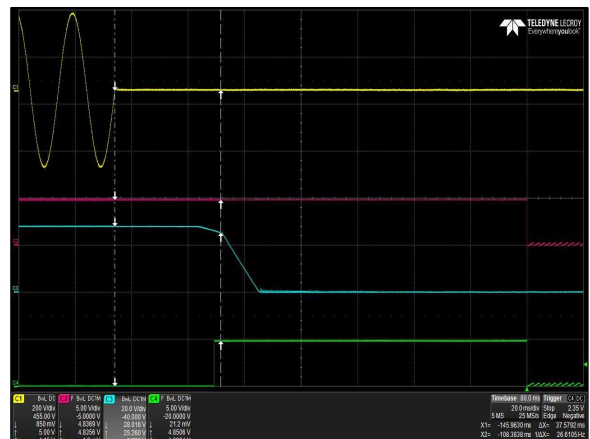
Figure 34: LCC600-28H-9P Hold-up Time
