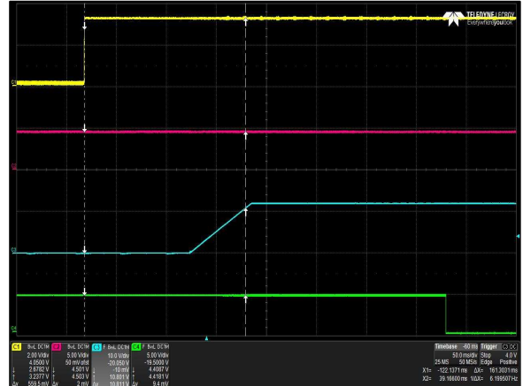
Figure 12: LCC600-12H-9P Turn-on delay via INH_EN
