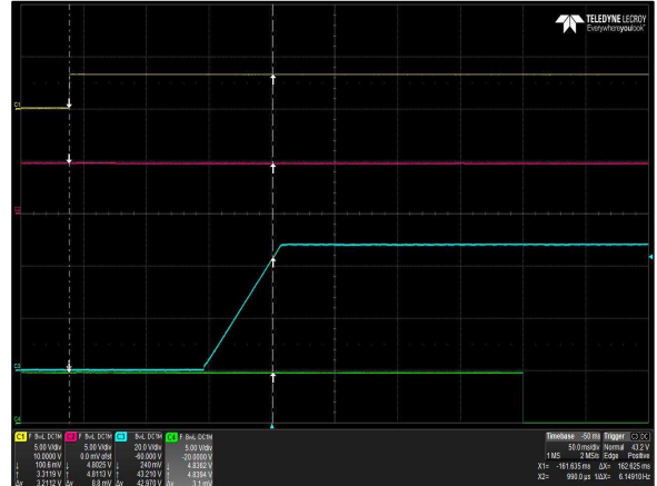
Figure 72: LCC600-48H-9P Turn-on delay via INH_EN
