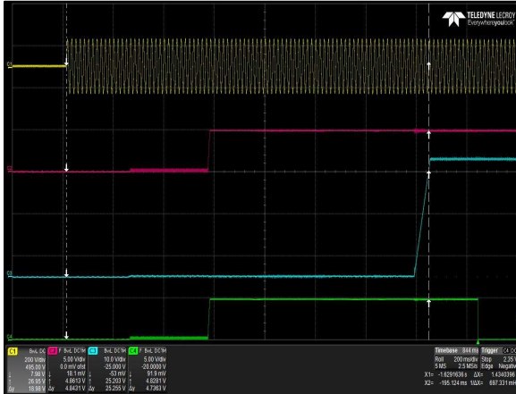
Figure 21: LCC600-28U-9P Turn-on delay via AC mains
