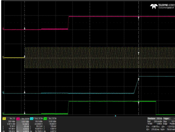
Figure 11: LCC600-12H-9P Turn-on delay via AC mains
