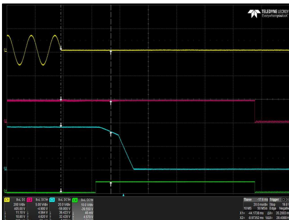
Figure 43: LCC600-36U-9P Hold-up Time
