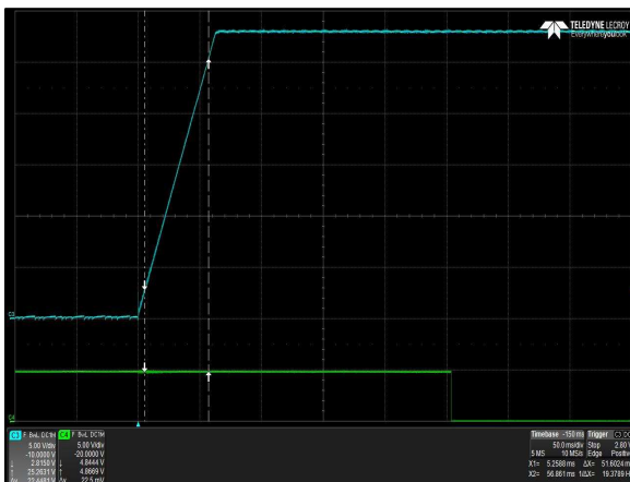
Figure 25: LCC600-28U-9P Output Startup Characteristic
