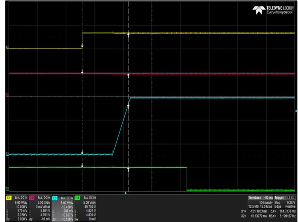
Figure 2: LCC600-12U-9P Turn-on delay via INH_EN
