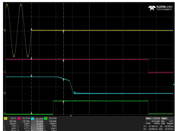
Figure 4: LCC600-12U-9P Hold-up Time
