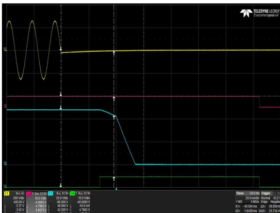
Figure 73: LCC600-48H-9P Hold-up Time
