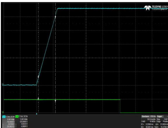
Figure 35: LCC600-28H-9P Output Startup Characteristic
