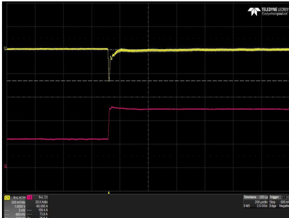
Figure 17: LCC600-12H-9P Transient Response - V_O Deviation 50% to 100% load change 1A/uS slew rate V_{in} = 277V_{ac} Ch 1: V_O Ch 2: I_O
