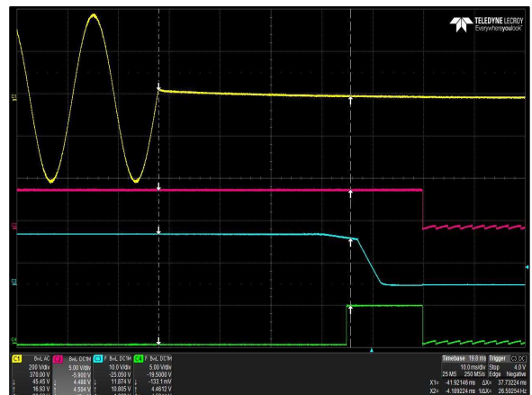
Figure 14: LCC600-12H-9P Hold-up Time
