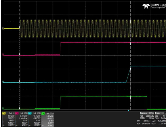
Figure 1: LCC600-12U-9P Turn-on delay via AC mains
