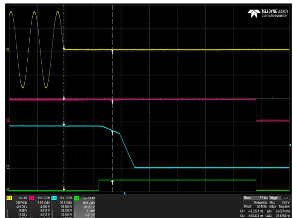
Figure 44: LCC600-36U-9P Hold-up Time
