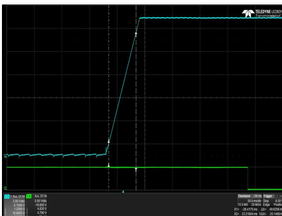
Figure 5: LCC600-12U-9P Output Startup Characteristic
