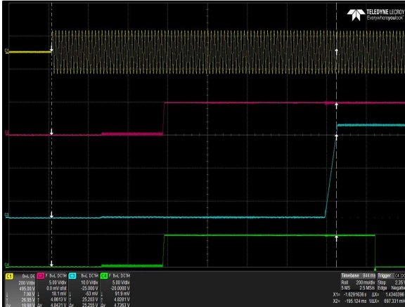
Figure 31: LCC600-28H-9P Turn-on delay via AC mains
