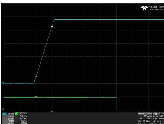
Figure 75: LCC600-48H-9P Output Startup Characteristic
