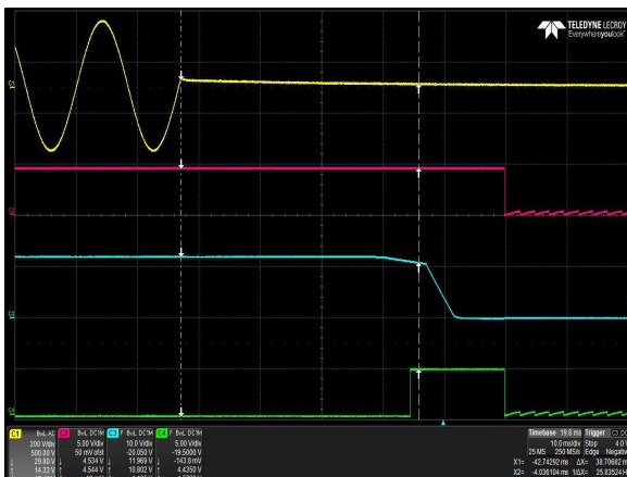
Figure 13: LCC600-12H-9P Hold-up Time
