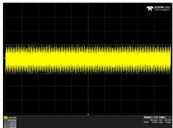
Figure 16: LCC600-12H-9P Ripple and Noise Measurement
