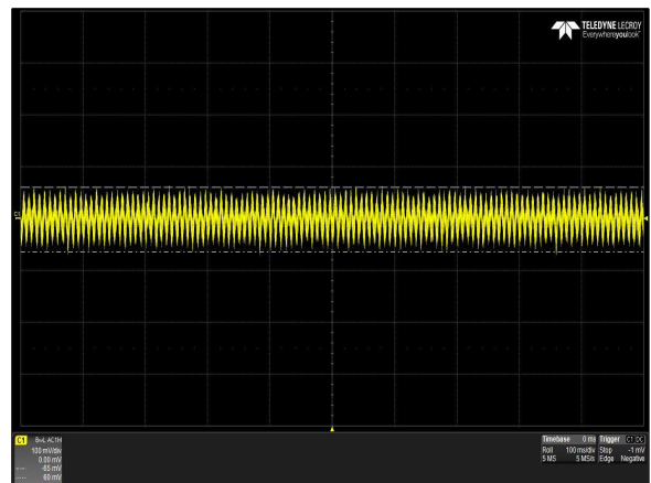
Figure 36: LCC600-28H-9P Ripple and Noise Measurement
