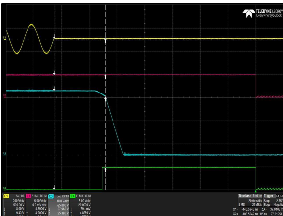
Figure 33: LCC600-28H-9P Hold-up Time
