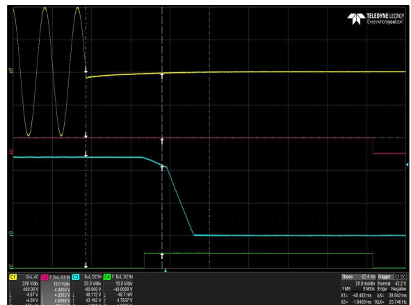
Figure 74: LCC600-48H-9P Hold-up Time
