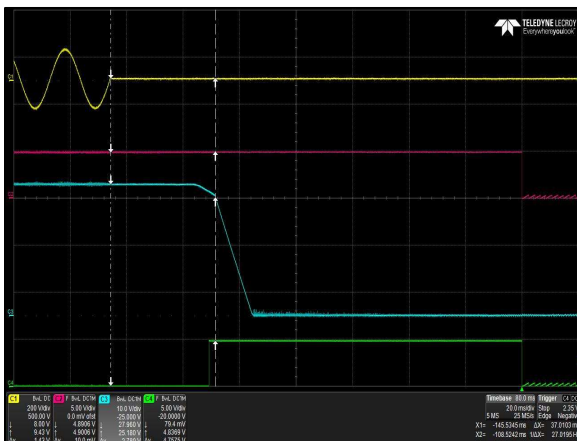
Figure 23: LCC600-28U-9P Hold-up Time
