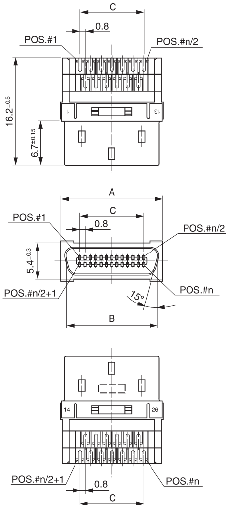
26-contact connector
