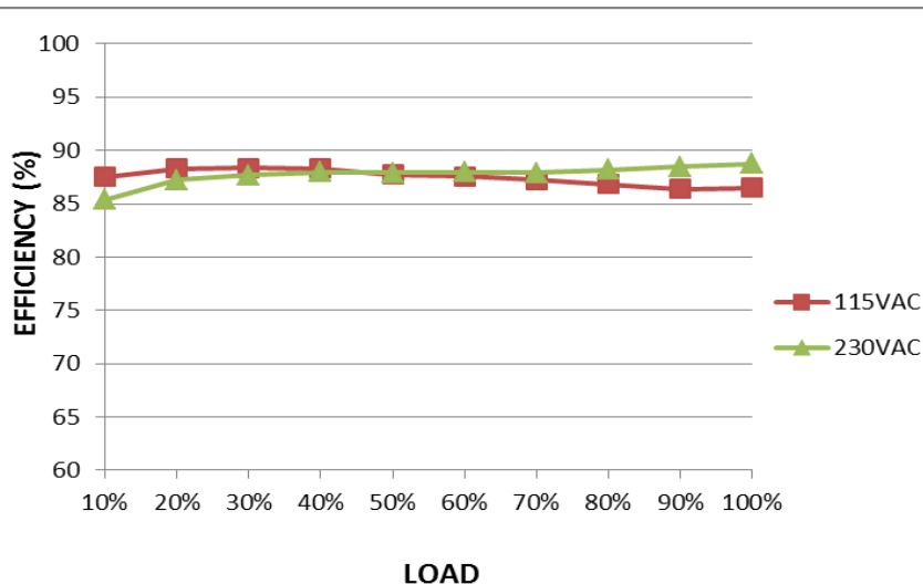
EFFICIENCY vs LOAD
