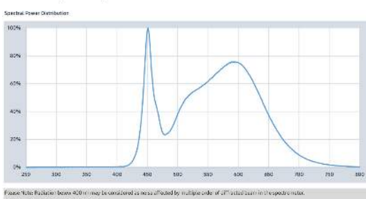
LM281B+, CRI80, 4000K
