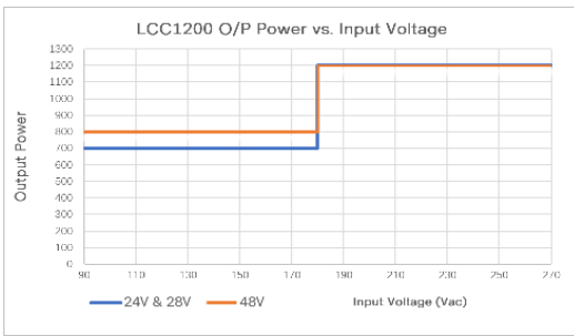
Figure 3. Output Power vs. Input Voltage
