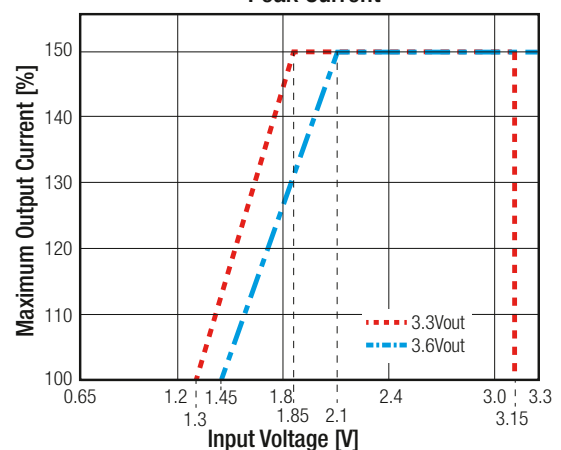
Peak Current
