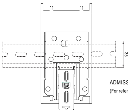
Back View
