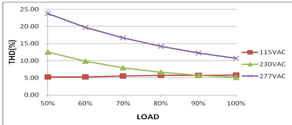
THD vs LOAD
