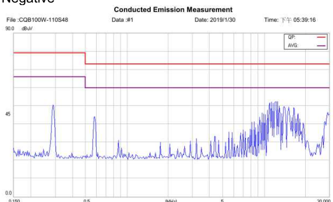
CQB100W-110S48-CMFC(D) Negative
