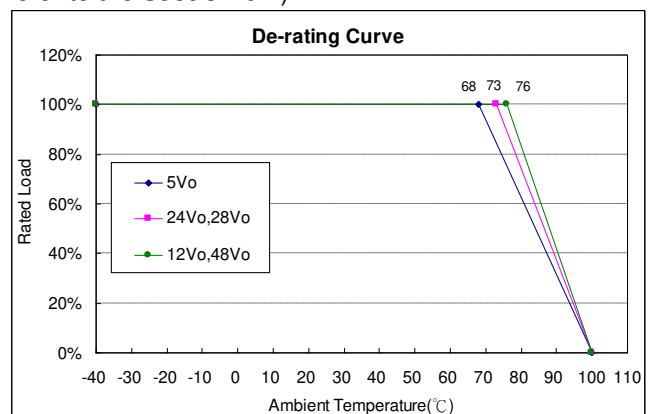
Ambient Derating Curves at Nominal Line, Full Load and Natural Convection, with heatsink (7.87x6.7x1.18inch)
