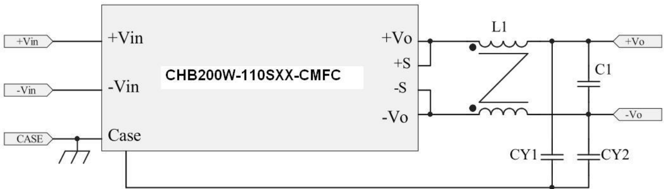
Connection circuit for EMI testing
