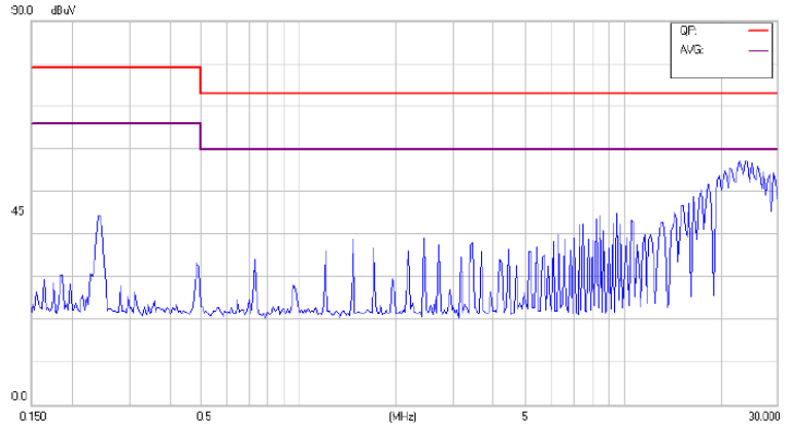
Conducted Class A CQB100W-48S15
