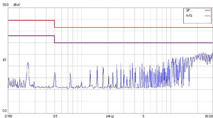
Conducted Class A of CQB100W-48S12
