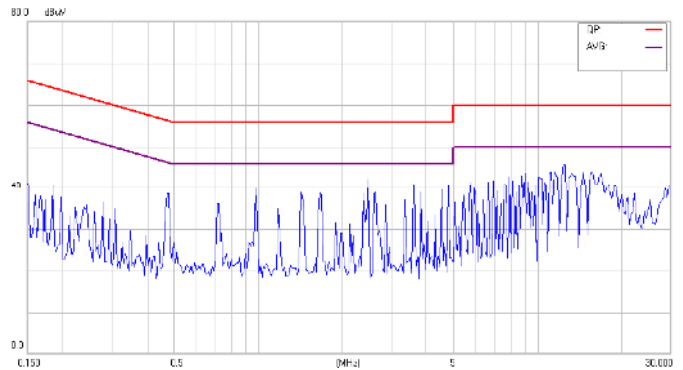
Conducted Class B of CHB150W-48S28
