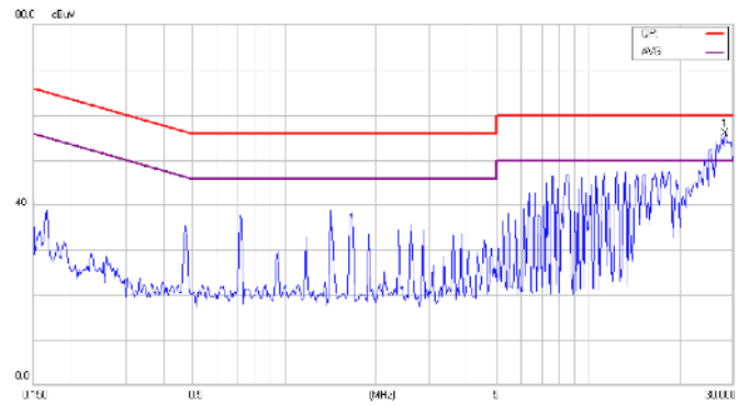
Conducted Class B of CHB150W-48S48
