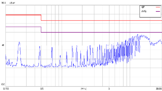
Conducted Class A of CHB150W-48S28
