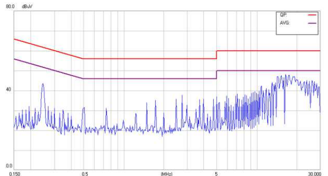
Conducted Class B of CHB150W-24S12
