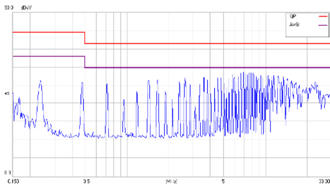
Conducted Class A of CHB150W-48S48
