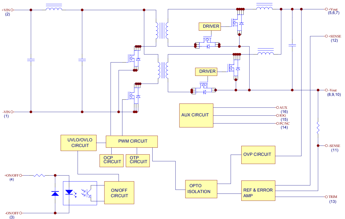
Electrical Block Diagram for 5V Modules
