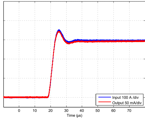
Figure 2: Typical delay time (0 to 300 A, 100 A/μs R_M = 10\ \Omega )
