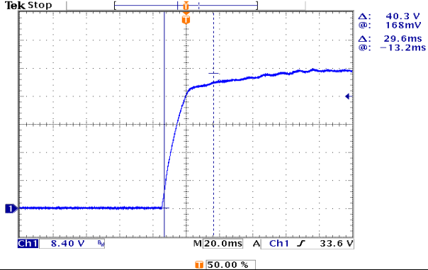
INPUT=230VAC/50HZ @ FULL LOAD CH1 : Output Voltage for V type
