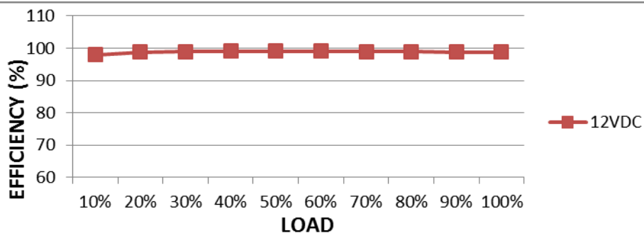
EFFICIENCY vs LOAD
